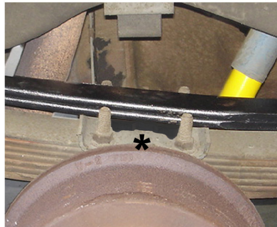
Atypical E350 Installation
