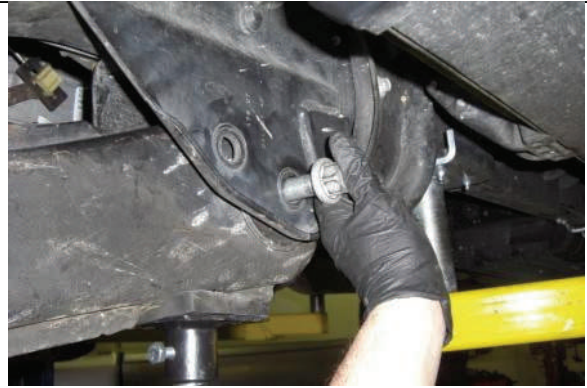
Support radius arm and remove attachment bolts
