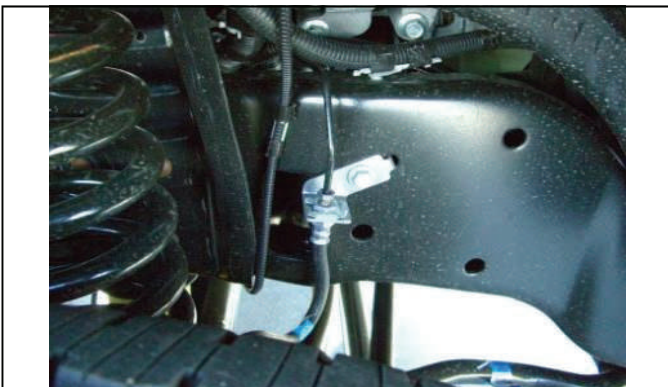
(08-10) models require drilling new 3/8 hole below OE hole.
